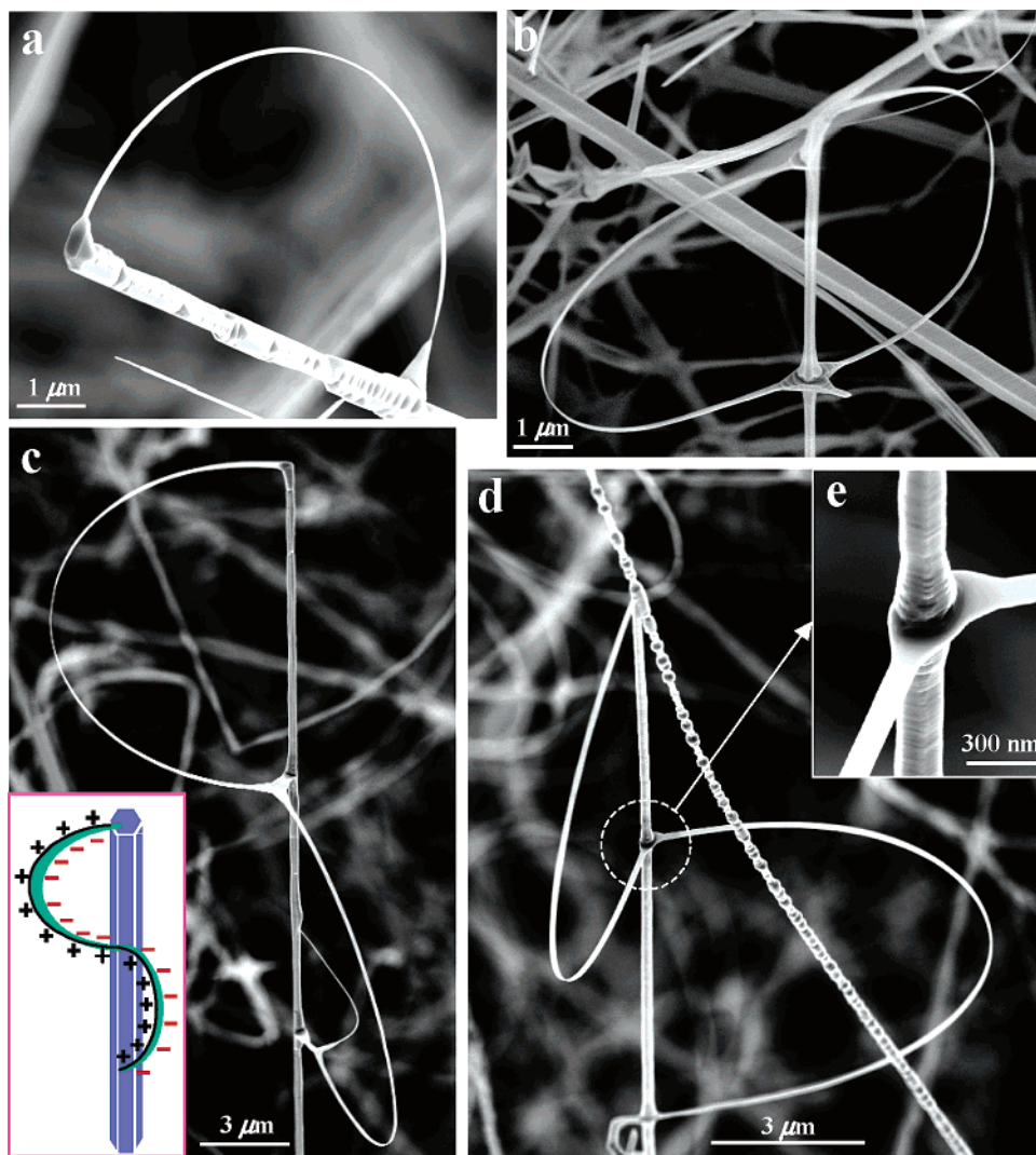
Figure 3. ZnO nanobows made from individual polar surface-dominated single-crystal nanobelts. A collection of typical geometrical shapes of the nanobows are presented. A model for the nanobow shown in (c) is inserted, showing their geometry and charge distribution along their polar surfaces (see text for details).
