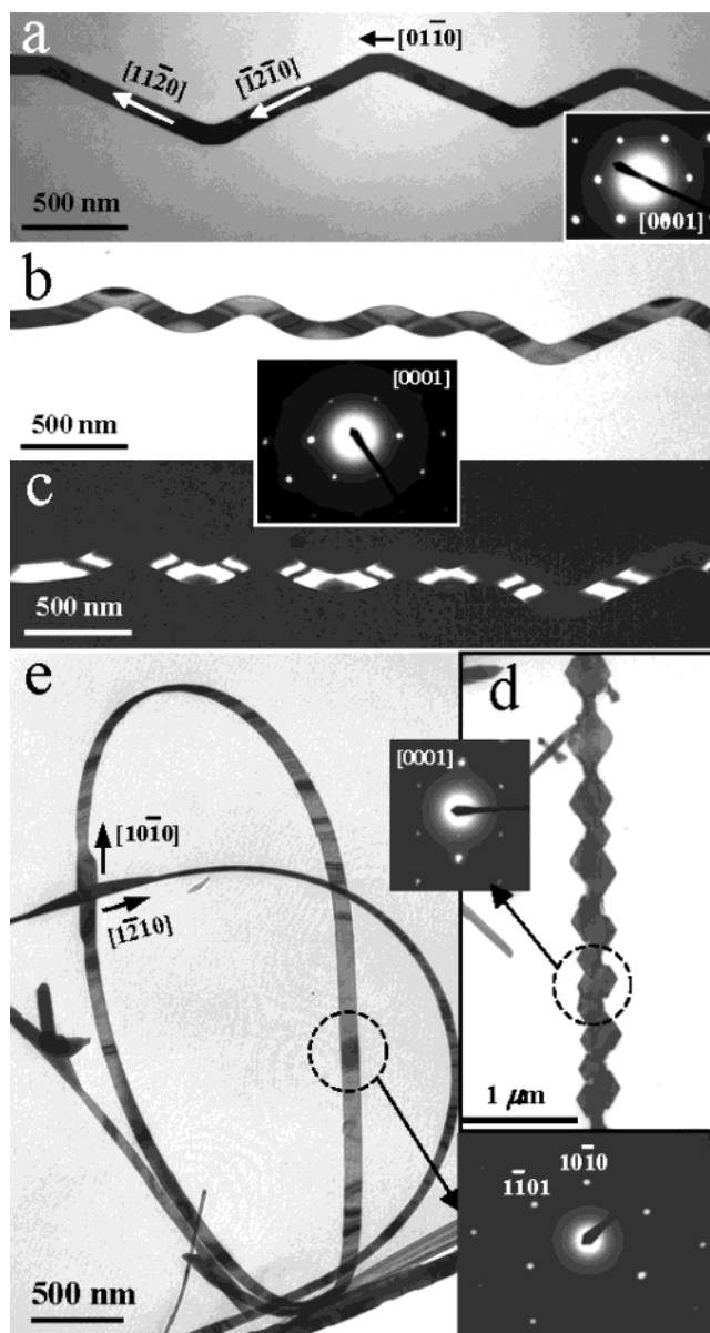
Figure 6. TEM images and their corresponding electron diffraction patterns for polar surface-dominated ZnO nanostructures with multiple growth directions. Changes in the growth directions are directly related to changes in the growth kinetics. (a,b) Single-crystal zig-zag, polar surface-dominated nanobelts alternating between their [11\bar{2}0] \rightarrow [01\bar{1}0] \rightarrow [\bar{1}2\bar{1}0] directions. (c) Dark-field image showing periodic contrast and therefore periodic strain within a polar surface-dominated nanobelt. (d) Single-crystal platelets of polar surface-dominated ZnO showing extreme switching in growth directions. (e) An example of two nanorings growing from the same junction and having two different growth directions.
